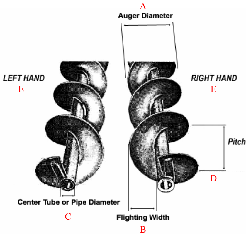
Right and Left Hand Screws
